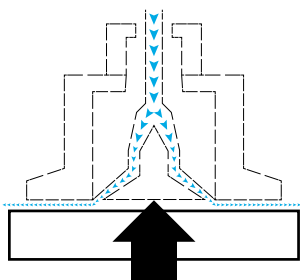
Bernoulli effect
